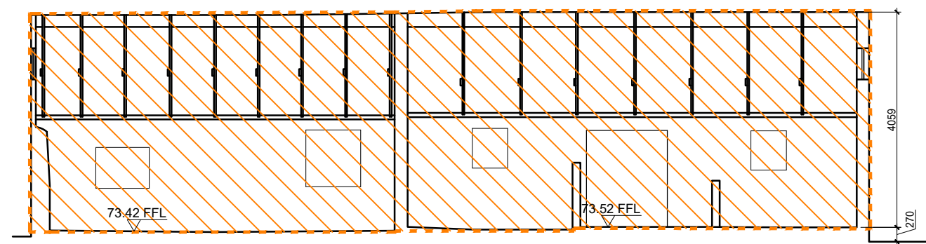
Existing Store Section A-A - DEMOLITION Scale 1:100 @ A3
